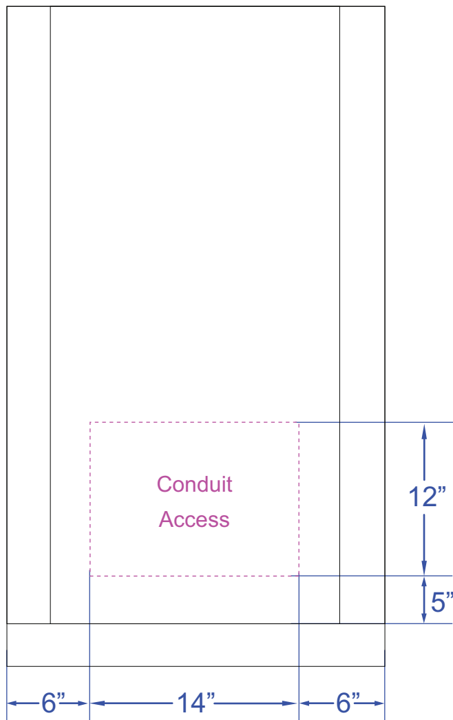
Right/Left Side View
